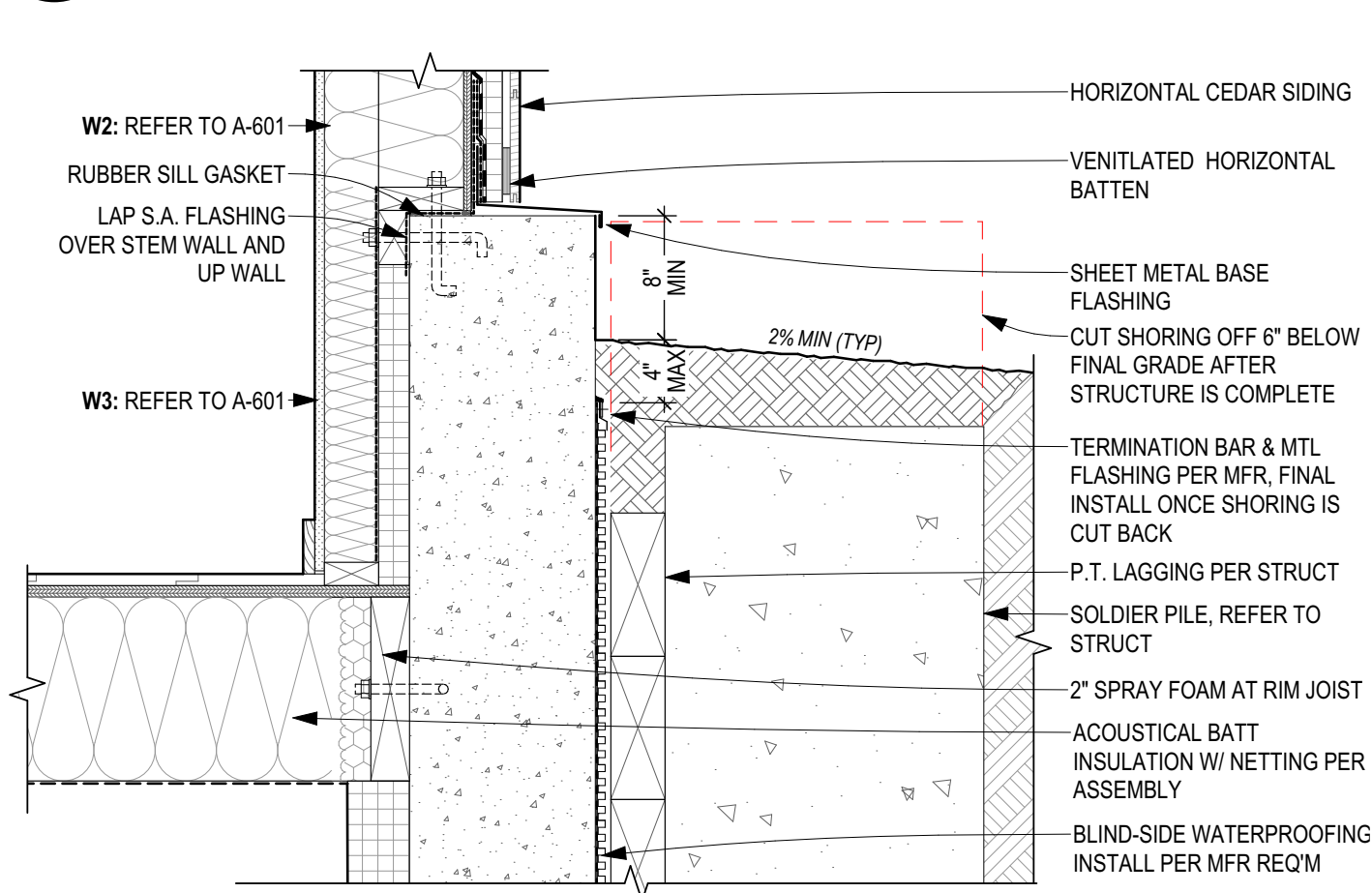
A2 TYP. WALL BASE AT SHORING SCALE: 1" = 1'-0"
