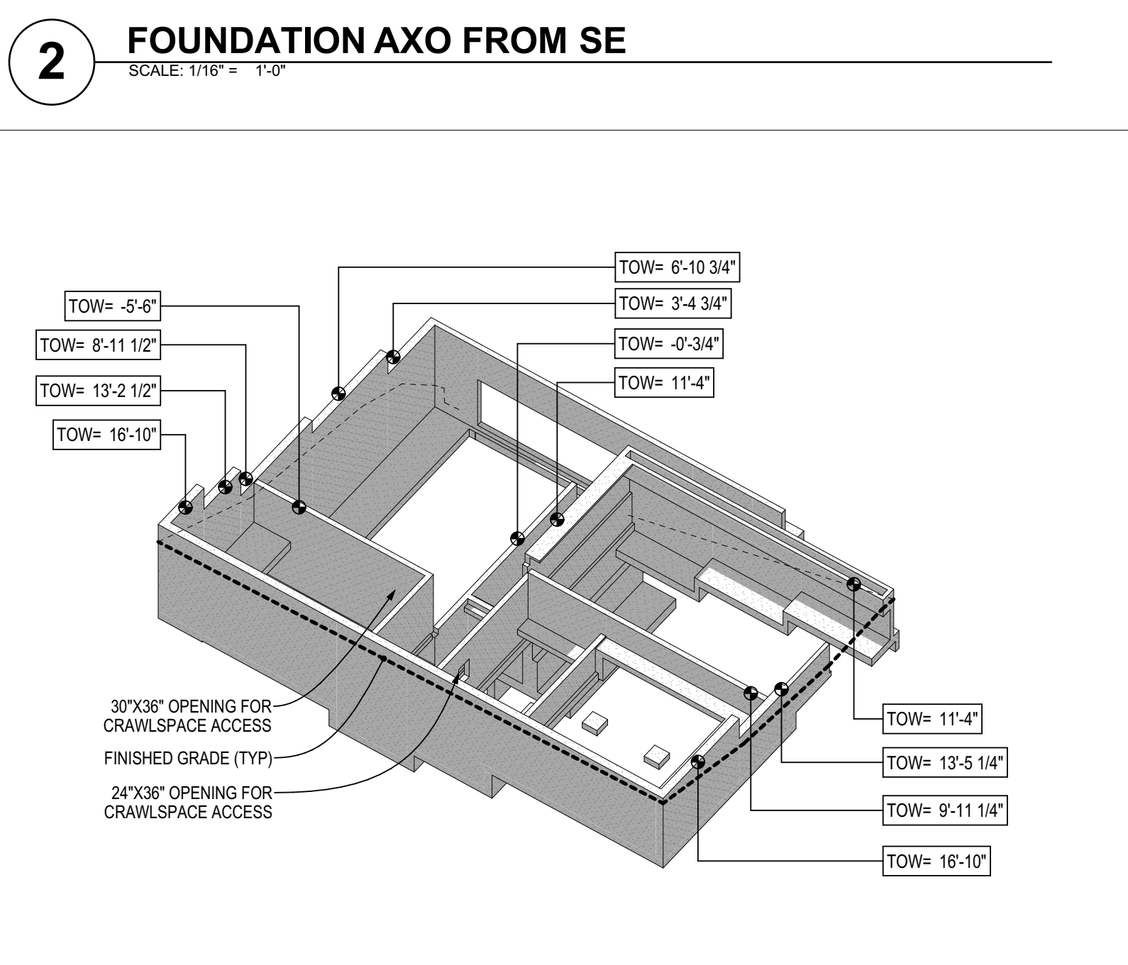
2 FOUNDATION AXO FROM SE SCALE: 1/16" = 1'-0"
